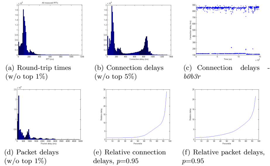
Fig. 2. Measurement results
